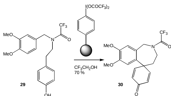
Scheme 13 Use of polymer supported PIFA 1 in the synthesis of oxomarithidine
