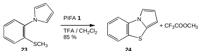
Scheme 10 Interrupted Pummerer reaction
